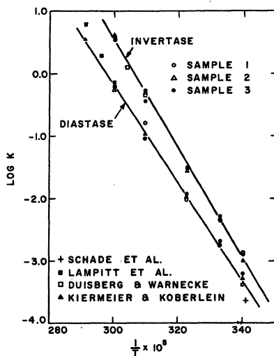
Fig. 1. Effect of temperature on rate of heat inactivation of diastase and invertase in honey. For diastase, \log k = 22.764 - \frac{35010}{2.303 ET} ; for invertase, \log k = 26.750 - \frac{39730}{2.303 ET}
